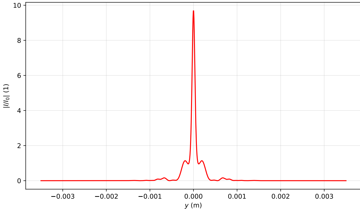
Intensity profile I(x=0, y, z=0.955)/I_0 , \text{Pin}=7.0\text{Pcr} , artificial time
